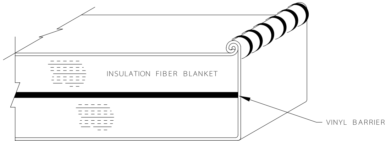
"ACCOUSTA - SET" CONSTRUCTION 140°F AND BELOW (AFTER 1" THK BLANKET)
