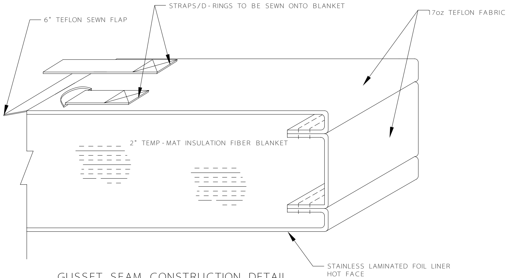
GUSSET SEAM CONSTRUCTION DETAIL
